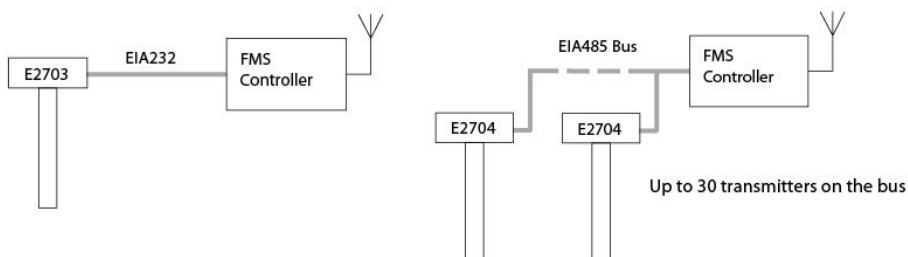
Connection diagrams
