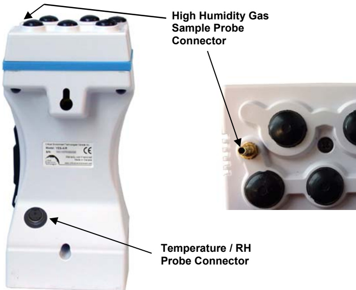
Figure 10-1. YESAIR for Dual-Probe Applications
