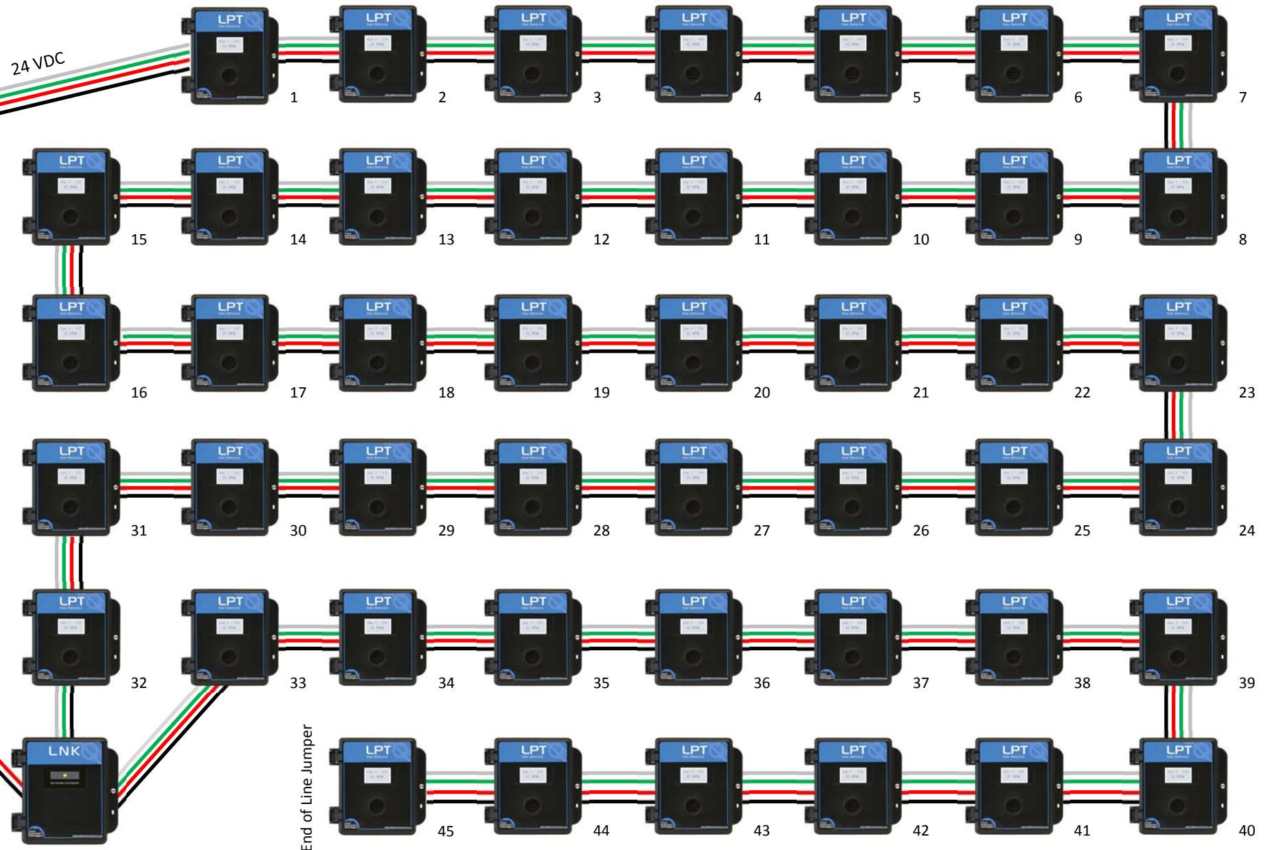
LNK-XT Network Extender installed every 609 m (2000 ft)
