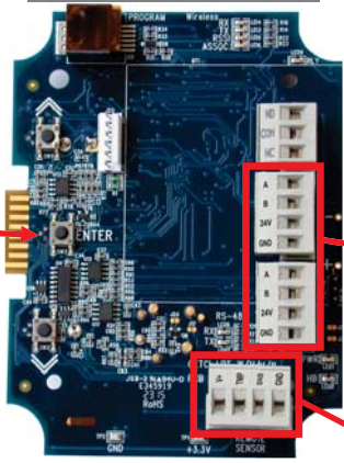
LPT-M CIRCUIT BOARD
