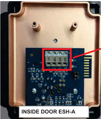
INTERNAL CATALYTIC COMBUSTIBLE (H 2 , CH 4 or C 3 H 8 )
