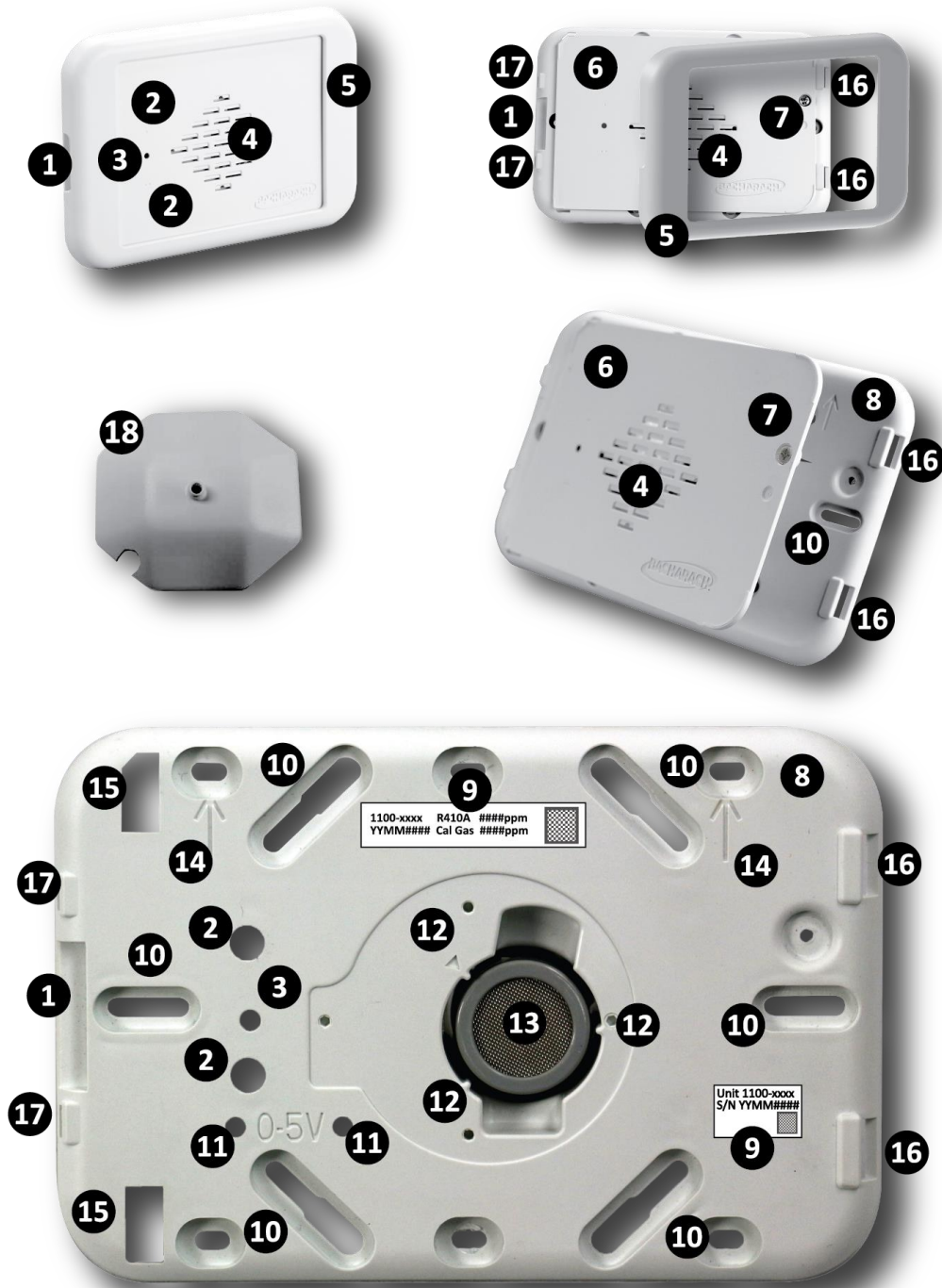
Figure 2. MVR-300 Components (Front)
